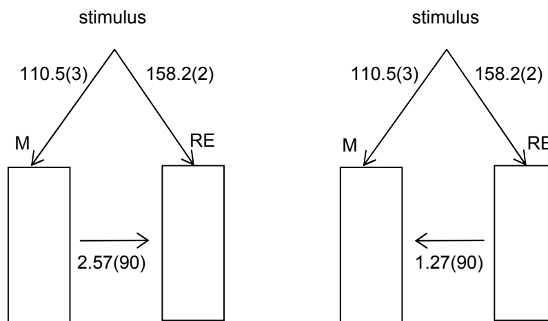
Figure 5. Estimates of the coefficients of mutual information for the links indicated. The integers in (·) are the degrees of freedom of the respective estimates.
