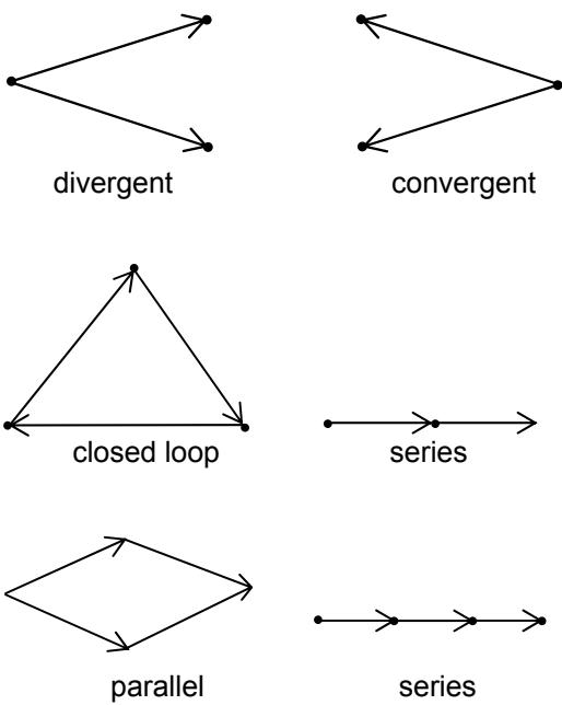
Figure 2. Some 3- and 4- node networks.
