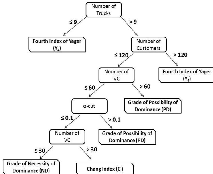
Figure 2: Decision tree model.
