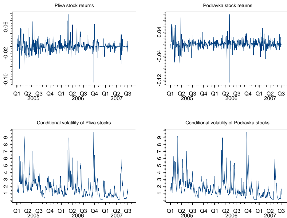
Figure 3: Returns of Pliva and Podravka stocks with their conditional volatilities
