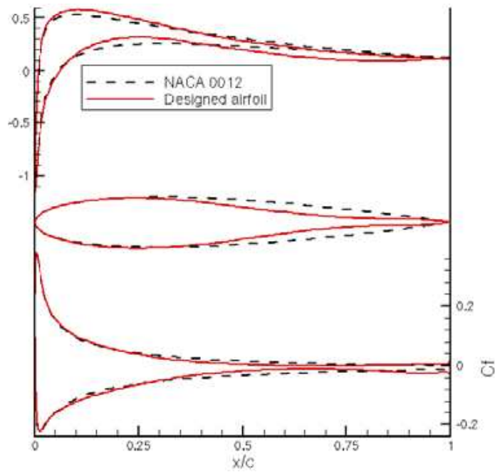
Figure 2. Initial and designed C_p and C_f
