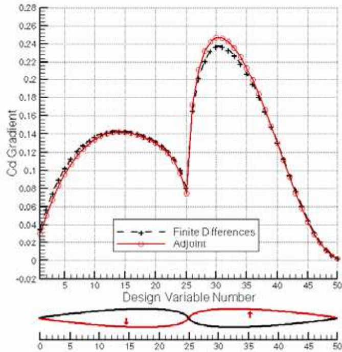
Figure 1. Viscous C_d subsonic gradients
