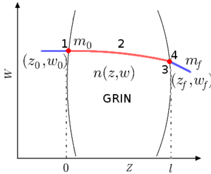
Figure 3 Schematic path of a light ray through the crystalline, showing the parameters to be measured and the steps of the calculation procedure.
