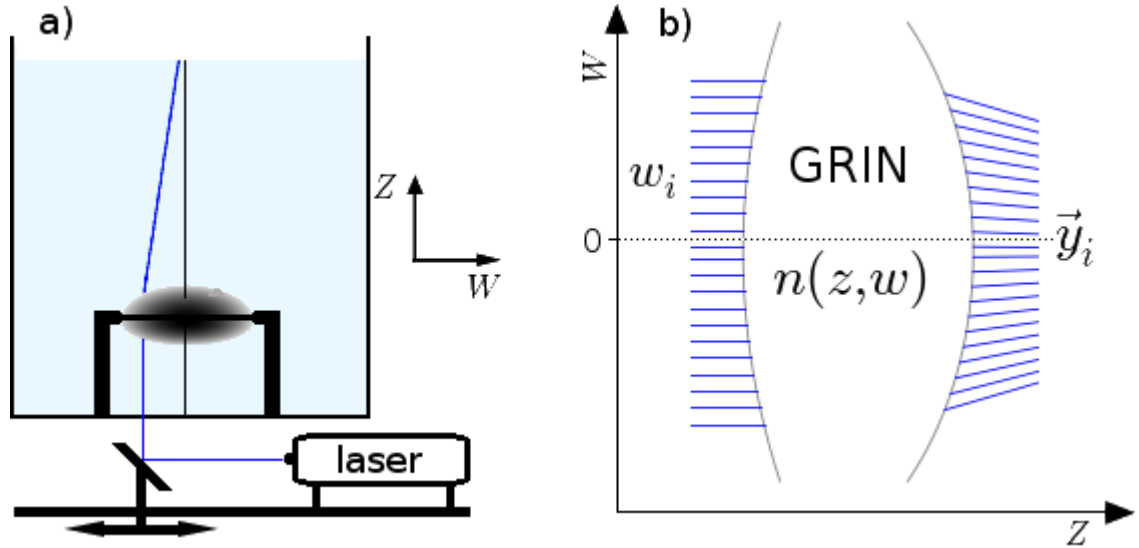
Figure 2 The experimental procedure. (a) Sketch of an experiment to measure ray paths before and after passing through the crystalline. (b) A set of measurements.
