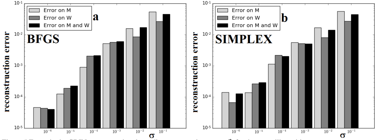
Figure 5 Errors in the GRIN reconstruction depending on errors in vectors \vec{y}_i for the crystalline with parameters taken from Table 1 (a) using BFGS, (b) using SIMPLEX. For each \sigma three bars are shown: light gray (left) considers only errors in the slope of the outgoing ray, gray (center) only considers the error in the position of the exit point, black (right) errors in both magnitudes.
