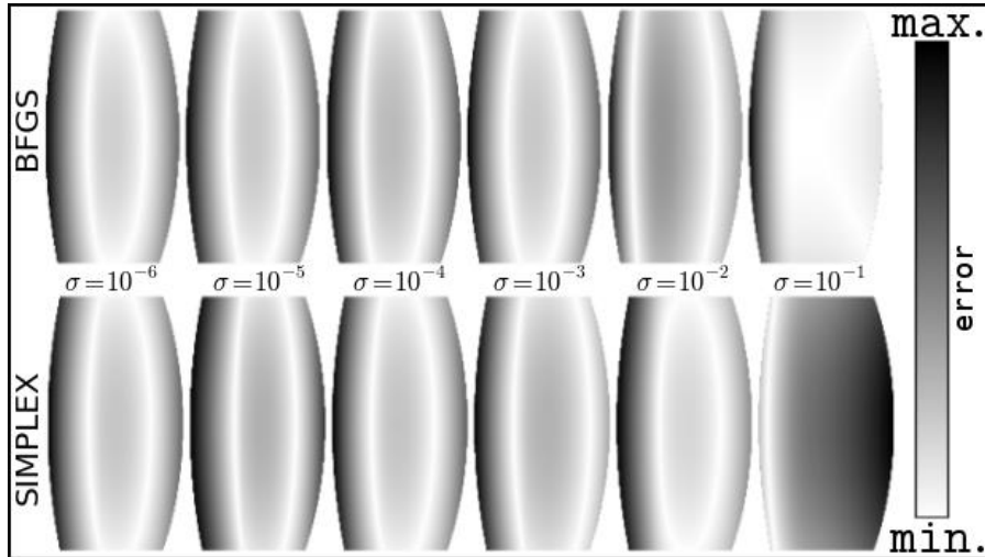
Figure 6 Spatial distribution of the absolute error in the GRIN reconstruction inside the crystalline. The scale shows relative values, see text.
