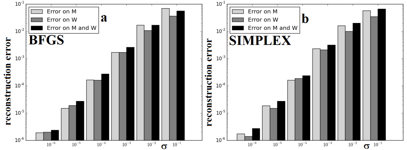
Figure 4 Errors in the GRIN reconstruction depending on errors in vectors \vec{y}_i for the crystalline with constant n = 1.42 (a) using BFGS, (b) using SIMPLEX. For each \sigma three bars are shown: light gray (left) considers only errors in the slope of the outgoing ray, gray (center) only considers the error in the position of the exit point, black (right) errors in both magnitudes.
